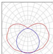
TRUST EVG PS 1 × 58W
