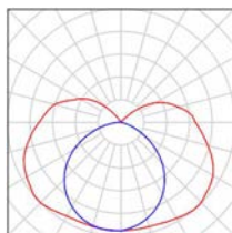
TRUST EVG PS 1 × 18W
