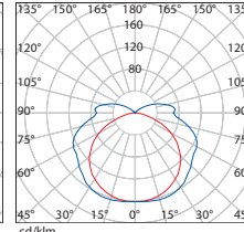
TRUST EVG PS 2 × 58W
